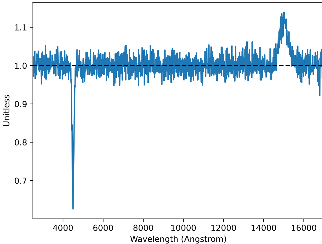
Continuum-normalized spectrum
