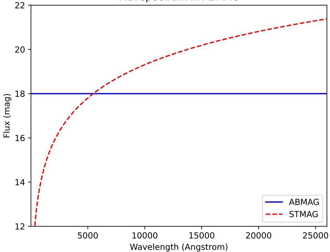
Flat spectrum in ABMAG
